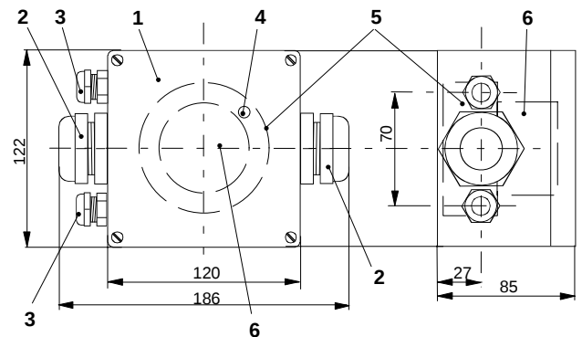
Fig. 1 Dimensioned drawing
